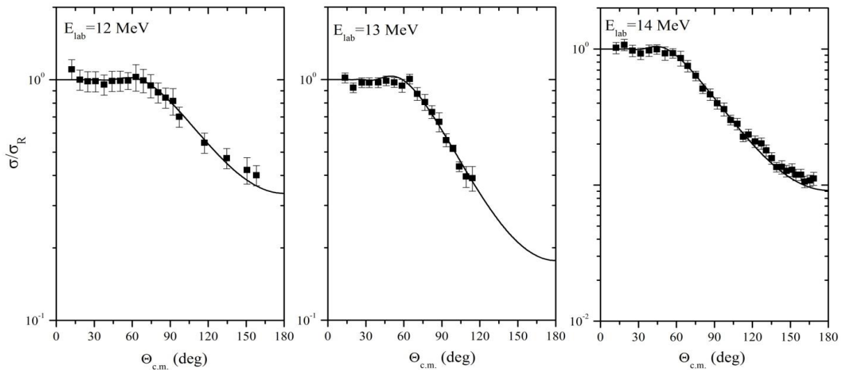
Figure 2 - The elastic scattering angular distributions for {}^9\text{Be}+{}^{28}\text{Si} at different energies. Points are the experimental data [23, 19], the solid line is the result of calculations using the double-folding potential with the parameters from Table 1.
