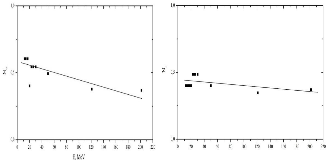
Figure 3 - The dependence of N_r and N_w on the energy of the incident nucleus.
