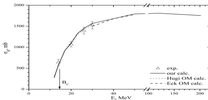
Figure 4 - Total reaction cross sections for the {}^9\text{Be} + {}^{28}\text{Si} interaction.
