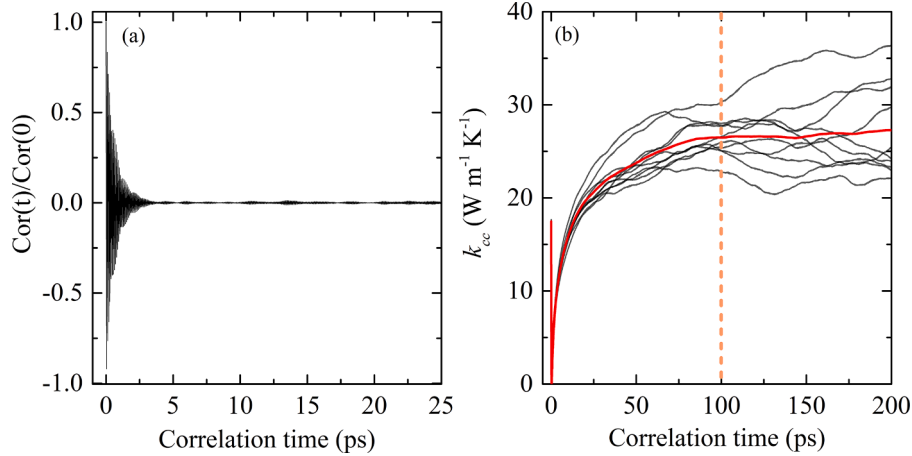
Fig. 8. (a) Correlation function dependence on correlation and simulation times from eq. (1) for the PCRM potential. (b) k_{cc} as a function of correlation time for different trajectories of atoms for the PCRM potential. The red line indicates the average k_{cc} value.
