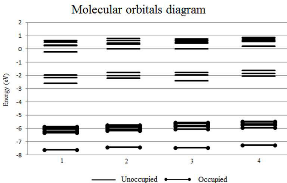
Figure 4. Diagram of molecular orbitals of the silicon clusters.
