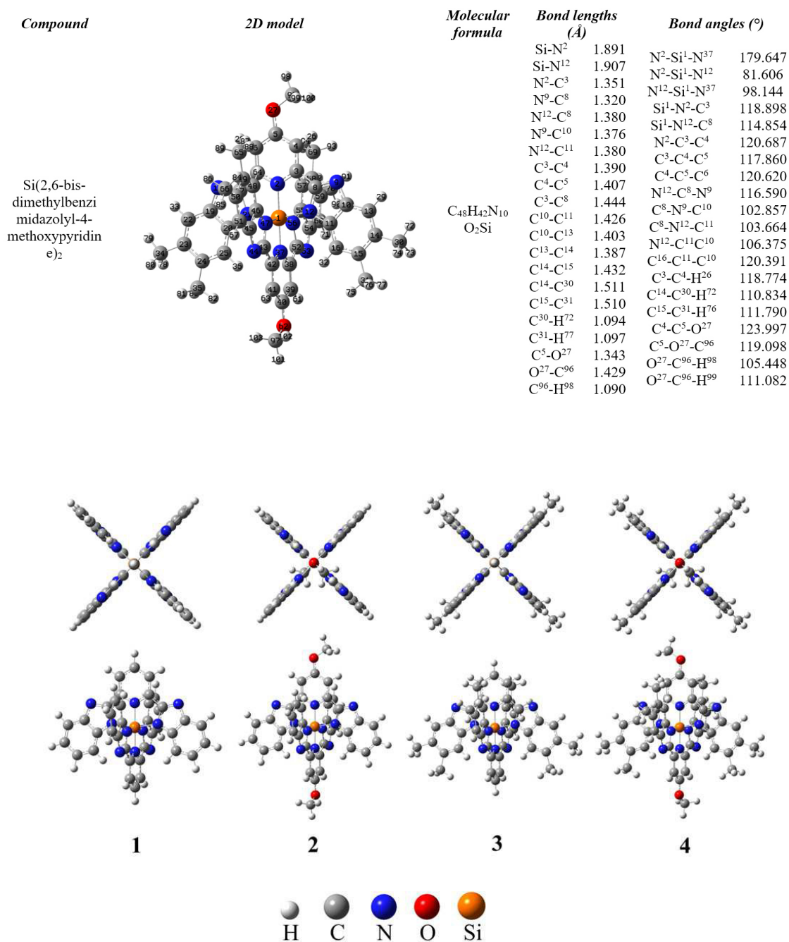
Figure 2. Optimized structures of nanoparticles.
