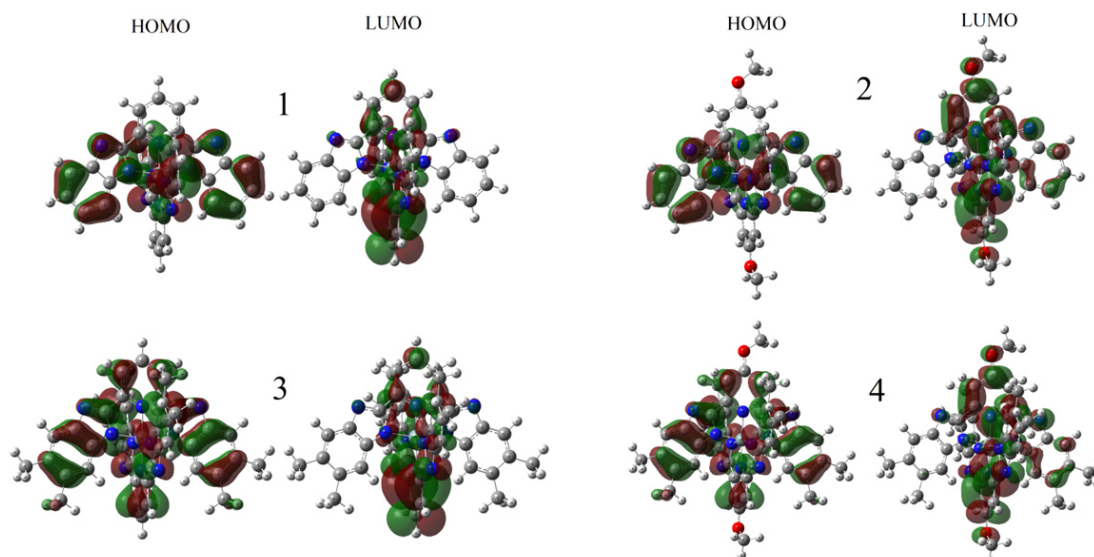
Figure 5. HOMO and LUMO of the complexes 1, 2, 3 and 4.
