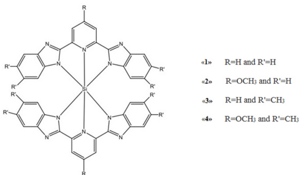
Figure 1. Chemical structure of observed types of hexacoordinate silicon complexes.
