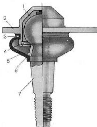
Figure 3. Direct load-bearing ball joint (a) and a variant of its modernization (b) using spring liners 1 – plastic insert; 2 – hinge body; 3 – spring ring; 4 – locking ring; 5 – rubber cover; 6 – spacer sleeve; 7 – hinge pin
