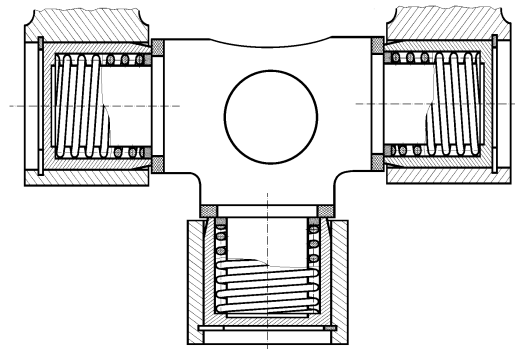
Figure 4. The upgraded crosspiece of the VAZ "Niva" car
