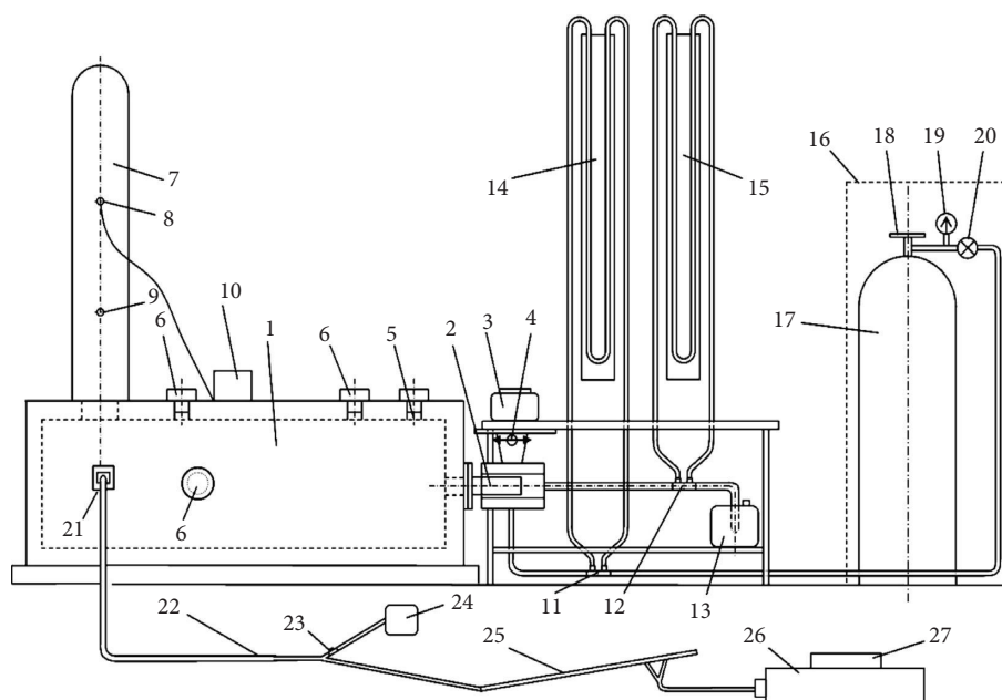
1 - combustion chamber; 2 - burner; 3 - autotransformer; 4 - device for burner moving; 5 - igniter; 6 - sight-holes; 7 - exhaust pipe; 8 - thermocouple; 9 - choke; 10 - millivtmeter; 11, 12 - flow rate washers; 13 - air flow switch; 14, 15 - fuel and air flow differential manometers; 16 - corps; 17 - gas cylinder; 18 - stop valve; 19 - manometer; 20 - flow regulator; 21 - sampling hatch; 22 - sampling line; 23 - shut-off valve; 24 - sample pump; 25 - sampling probe; 26 - gas analyzer; 27 - control module
