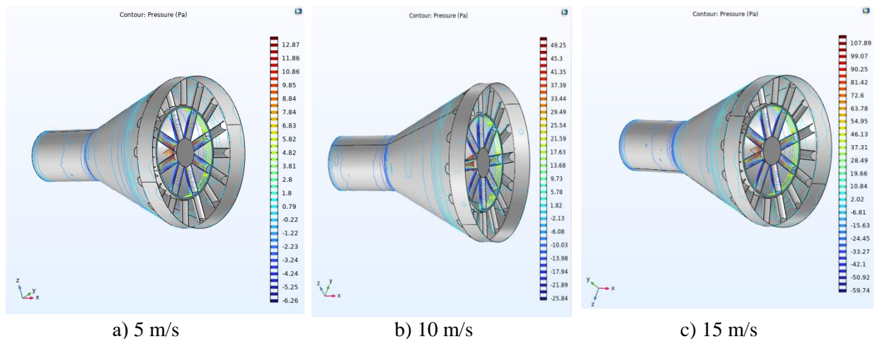
Figure 7. Pressure contours
